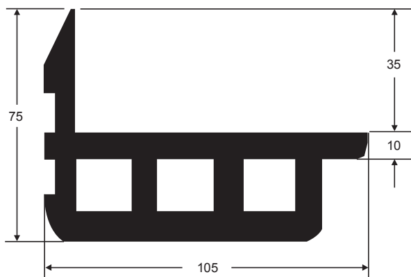
DR 1153* PONTOON BUFFER (available in custom lengths)
