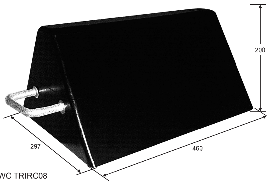
MOULDED LARGE WHEEL CHOCK
